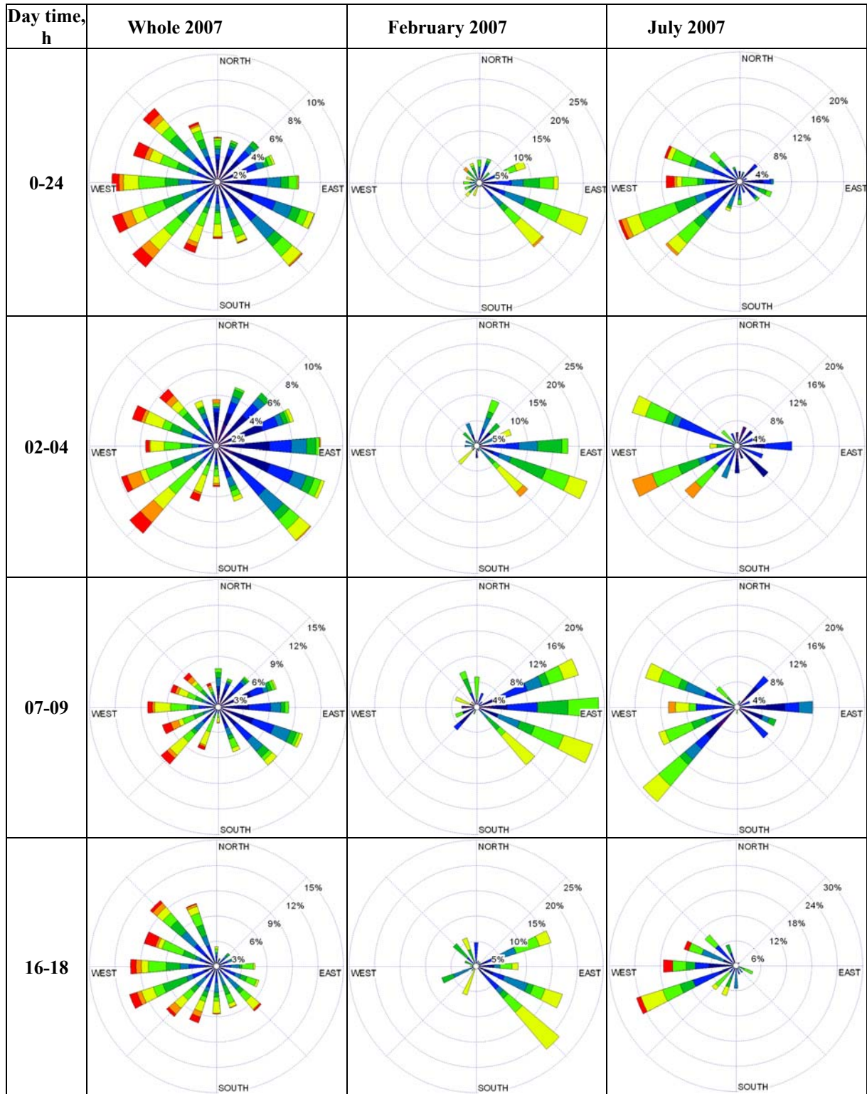
Fig. 3 Windroses during whole 2007, February 2007 and July 2007.
