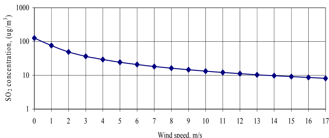
Fig. 7. SO 2 concentration in a monitoring station in accordance with CALPUFF, when one-way but different speed winds ( \mu\text{g}/\text{m}^3 ) are blowing
