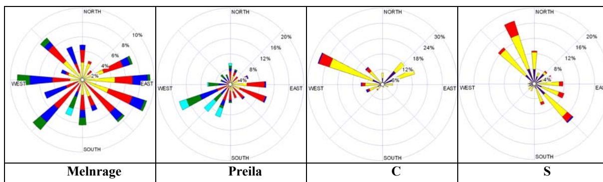
Fig 2. Windroses simultaneously recorded in the area of 4 monitoring stations during 6 weeks period.
