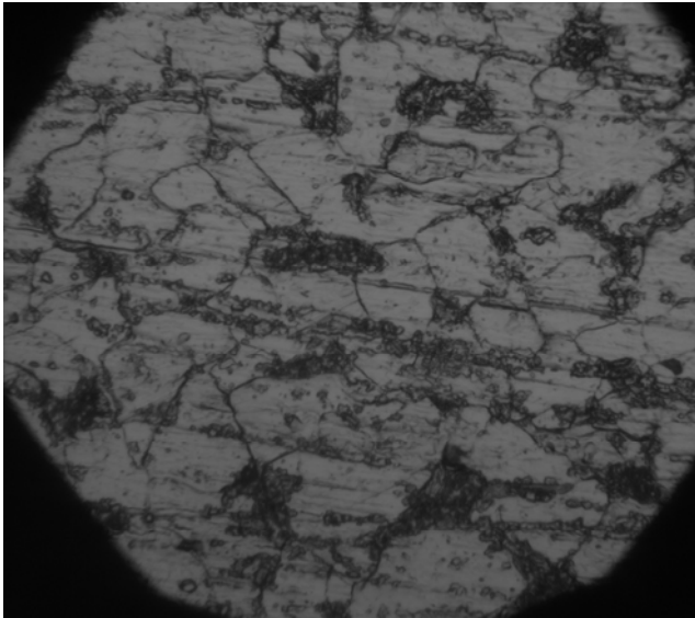
Fig. 7 An enlarged view (400 times) of materials micro-structure
