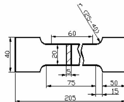
Fig. 1 Geometrical parameters of specimens used for tensile test
