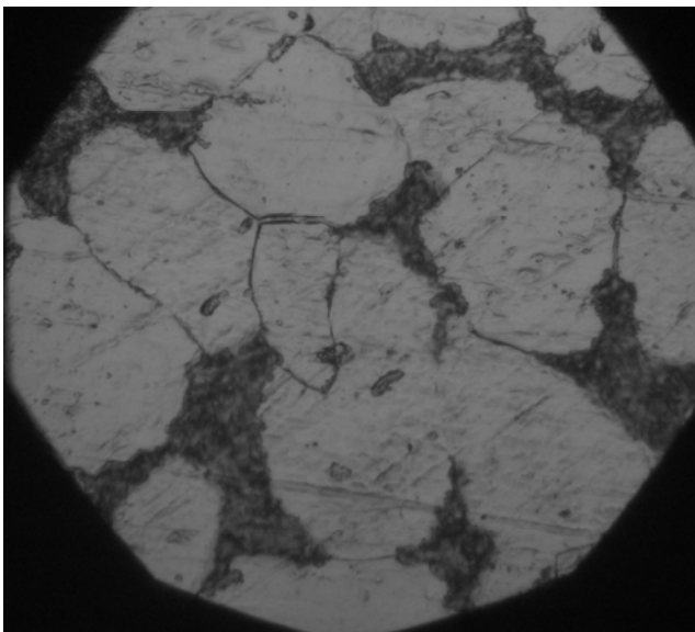
Fig. 8 An enlarged view (400 times) of materials micro-structure (in the case of brittle fracture)
