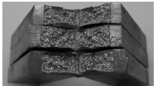
Fig. 6 Specimens after impact test (brittle fracture)
