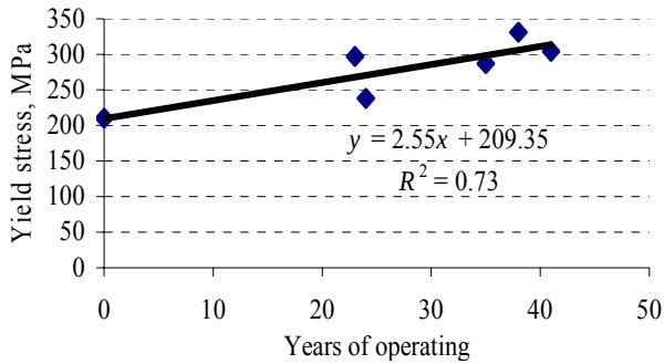
Fig. 2 Relationship between yield stress of materials and operating time
