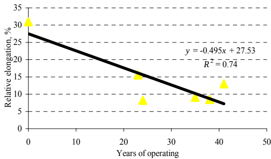
Fig. 3 Relationship between relative elongation and operating time
