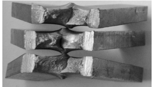
Fig. 5 Specimens after impact test (plastic fracture)
