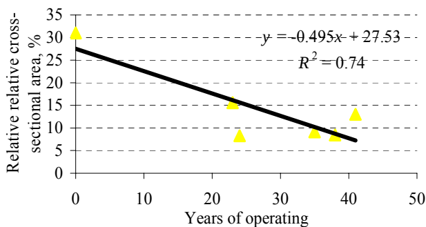
Fig. 4 Relationships between relative reduction of cross-section area and operating time
