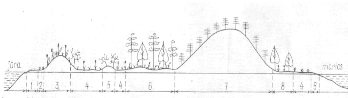
Fig 2. Ideal transverse profile of protective dune on the Curonian spit seashore (Bandžiulienė R.). 1. Sea beach; 2 – fore dune; 3 – coastal protective dune; 4 – plain beyond coastal dune; 5 – 6 hummock; 7 – biggest dunes; 8 – at the foot of biggest dune; 9 – beach of the Curonian lagoon.
