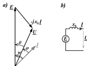
Fig. 1. Phasor diagram (a) and equivalent circuit (b) for the non-salient pole synchronous generator
