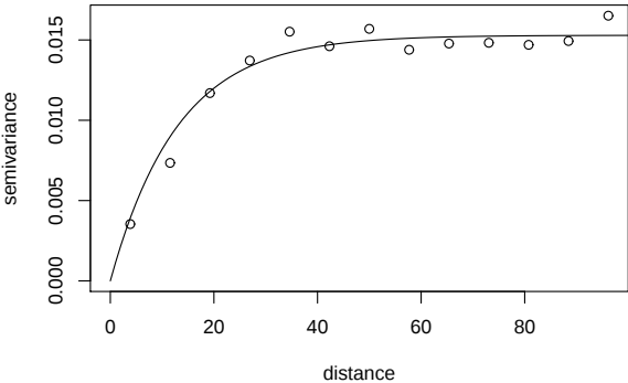
Fig. 2. Exponential semivariance model best fitted to the experiment data.
