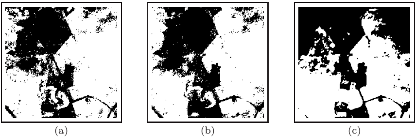
Fig. 3. (a) Classification results for PBDFD, (b) and PBDFI, (c) methods using 12 nearest neighbour scheme and method based on GLCM.
