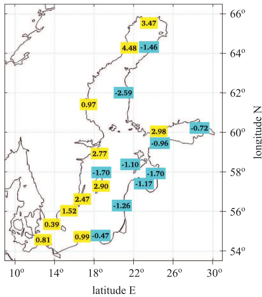
Figure 11. Trend of upwelling-favourable wind conditions [% decade -1 ] May–September (1990–2009) based on wind station data
