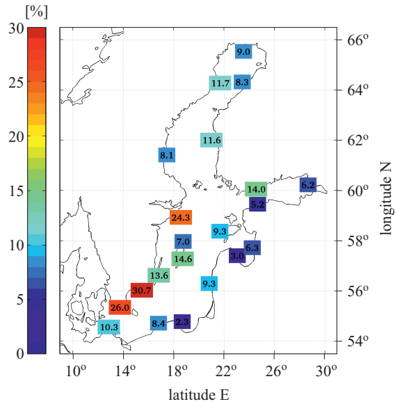
Figure 8. Frequencies of favourable wind conditions forcing upwelling [%] for the months of May–September for the period 1990–2009
