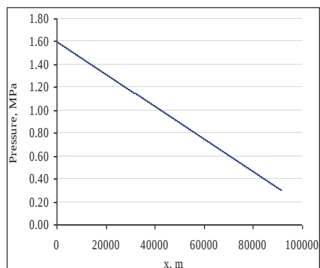
Fig. 7. Initial pressure distribution in the pipeline
