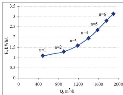
Fig. 17. Comparative energy dependence on oil pipeline productivity
