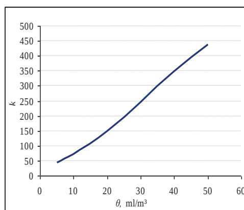
Fig. 4. Dependence of coefficient k on the FLO-XL additive concentration
