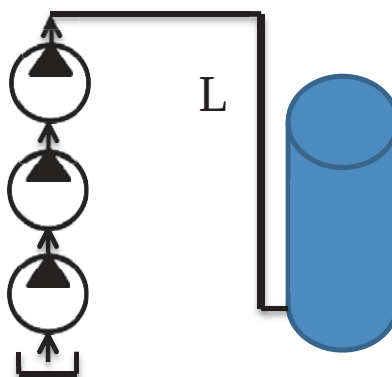
Fig. 2. Hydrodynamics system
