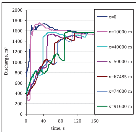
Fig. 11. Dependencies of the discharge in the different pipeline points when the concentration of the additives in the oil is equal to 12 ml/m³
