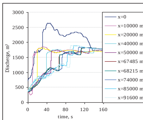
Fig. 13. Dependencies of the discharge in the different pipeline points when the concentration of the additives in the oil is equal to 50 \text{ ml/m}^3
