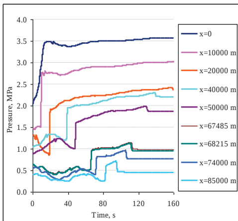
Fig. 10. Dependencies of the pressure in the different pipeline points when the concentration of the additives in the oil is equal to 12 ml/m³
