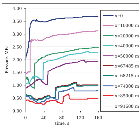
Fig. 8. Dependencies of the pressure in the different pipeline points when concentration of additives in the oil is equal 0 ml/m³
