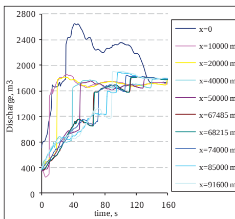
Fig. 9. Dependencies of the discharge in the different pipeline points when concentration of the additives in oil is equal 0 ml/m³
