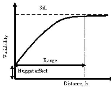
Fig. 1. Semivariogram representation.
