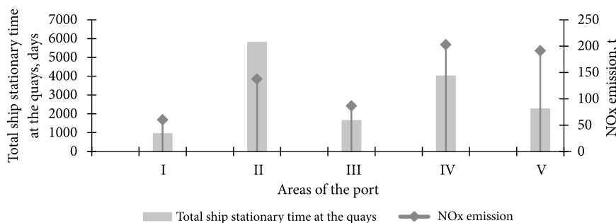
Fig. 4. Dependency between total ship stationary time at the wharves and NO x emission from the ships
