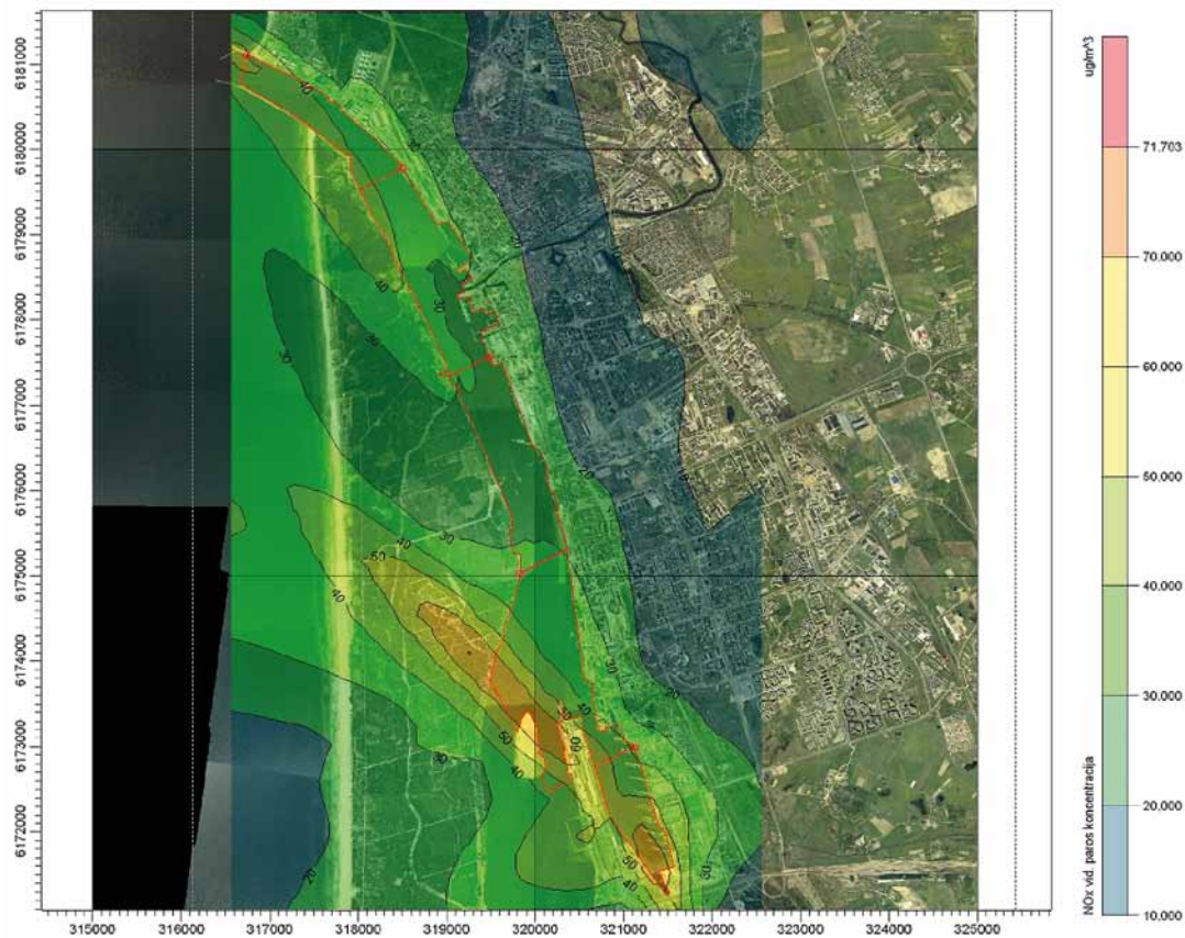
Fig. 7. Average daily concentrations of NO x (µg/m 3 ) due to emissions from ships in December
