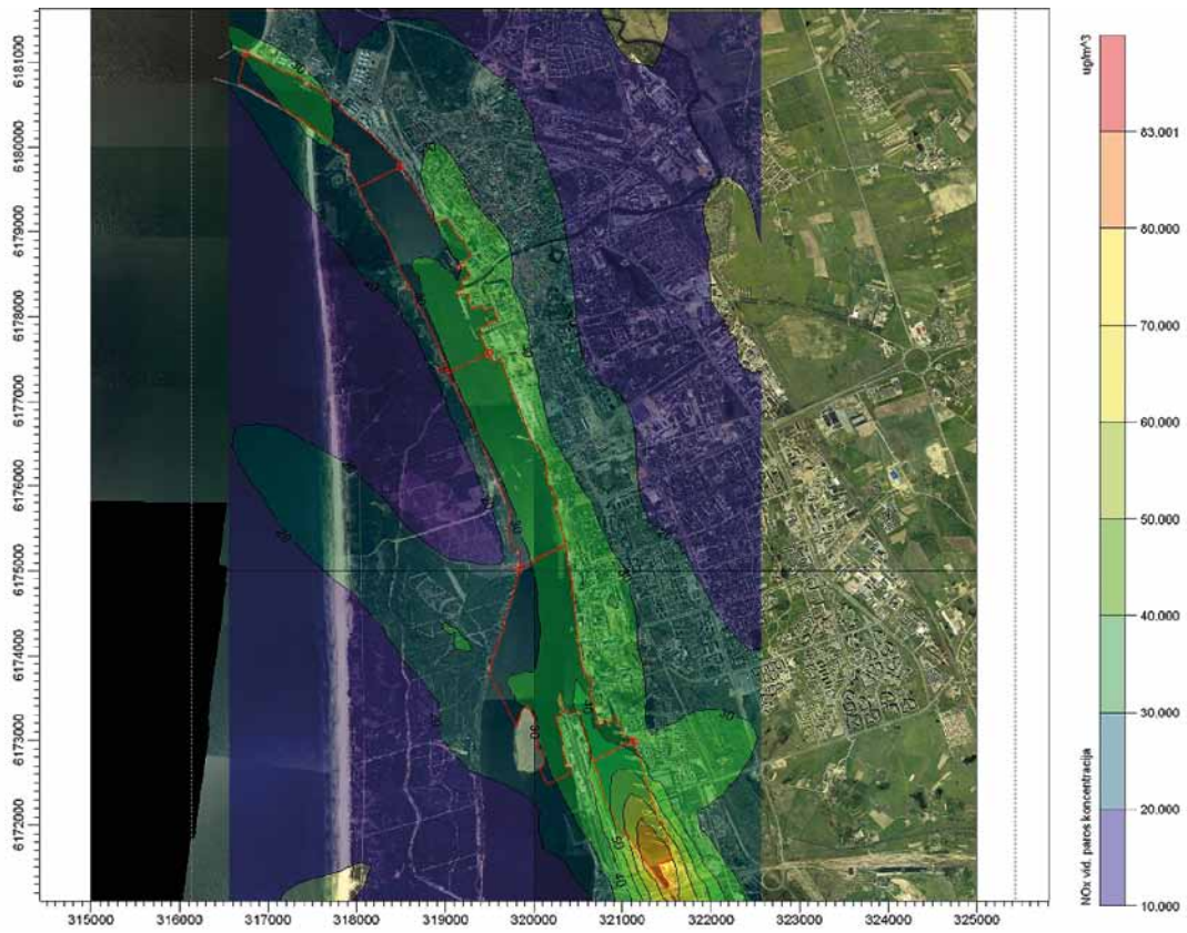
Fig. 6. Average daily concentrations of NO x (µg/m 3 ) due to emissions from ships in August
