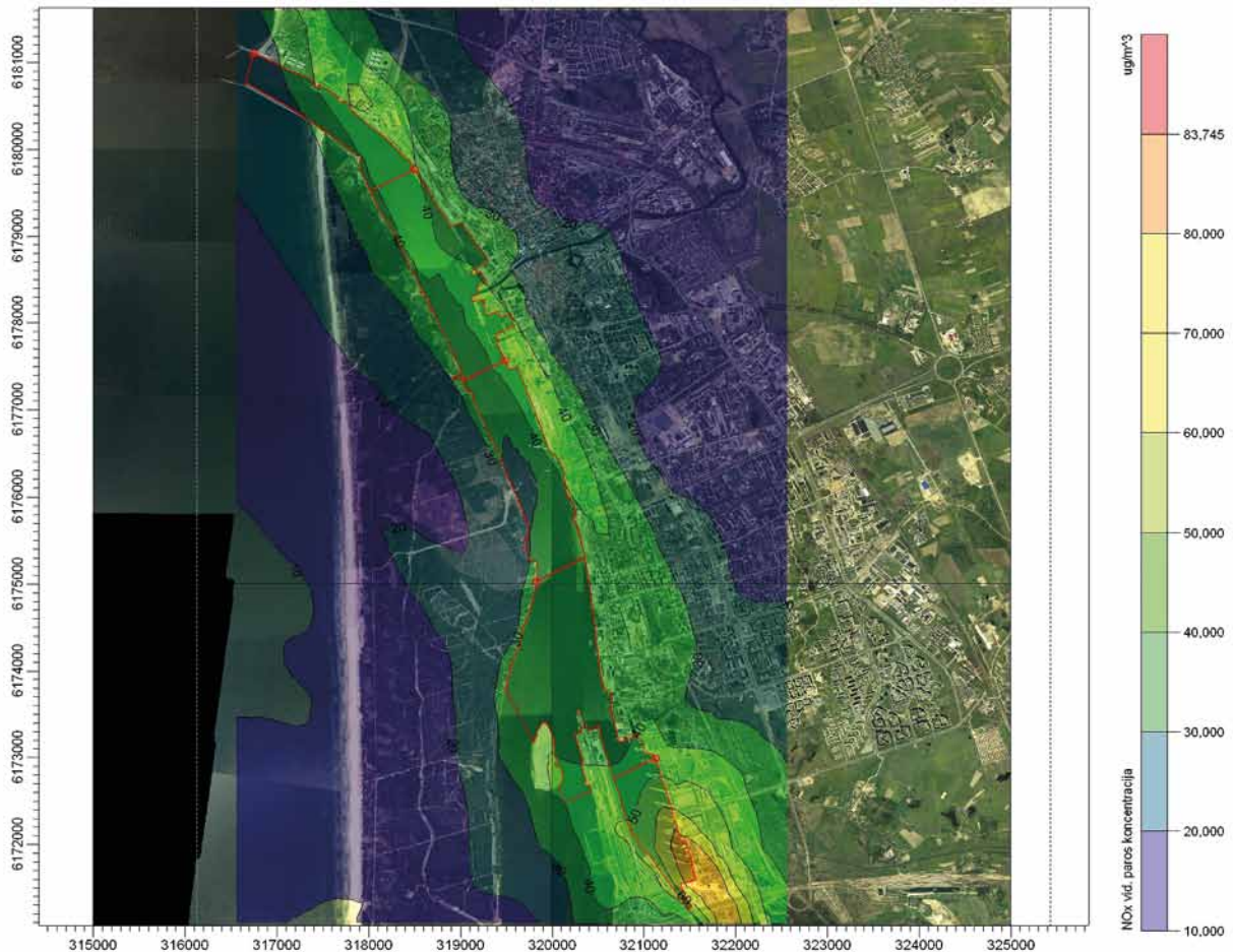
Fig. 5. Average daily concentrations of \text{NO}_x ( \mu\text{g}/\text{m}^3 ) due to emissions from ships in April
