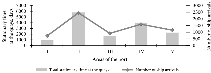
Fig. 3. Relation between number of ship arrivals and their total stationary time at the quays
