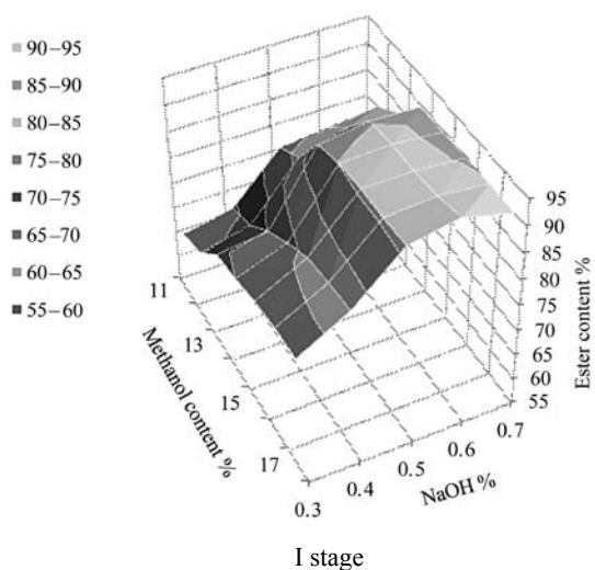
Figure 4. Influence of catalyst concentration and methanol content on false flax ( Camelina sativa ) oil methyl ester yield
