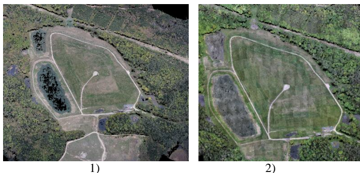
Fig. 4. Kariotiškės landfills territories digital surface model: 1) in year 2015; 2) in year 2016.
