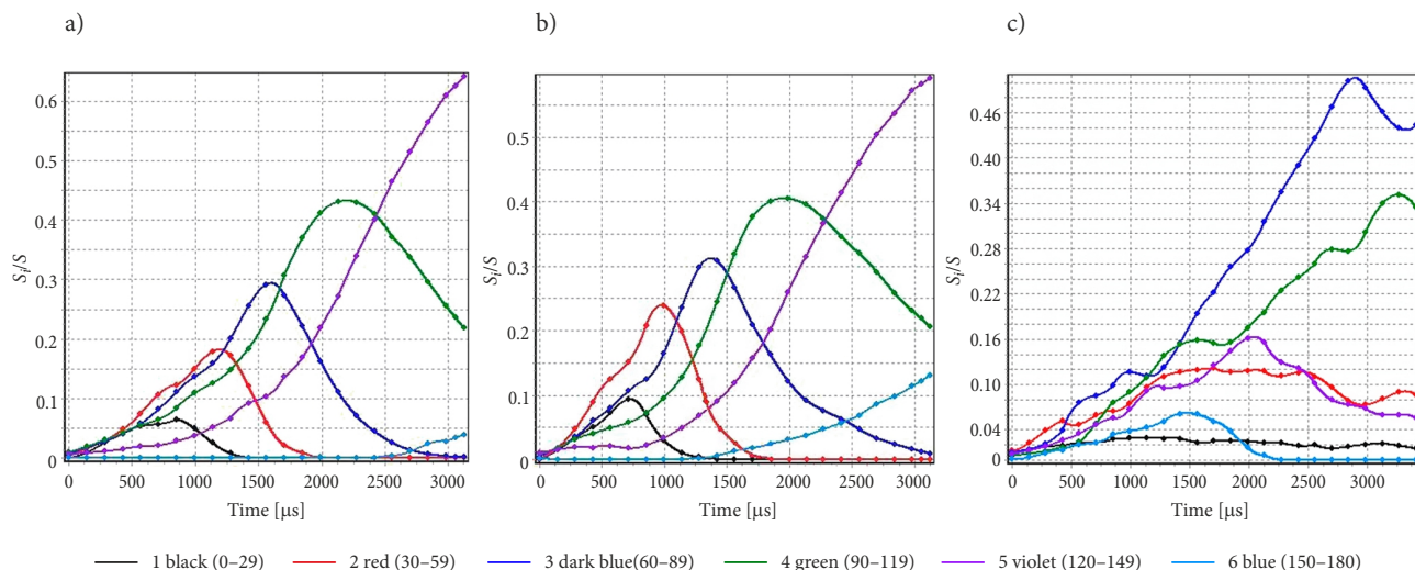
Figure 4. The structure of the fuel jet: a – CR system (60 MPa); b – CR system (100 MPa); c – CDS system (26°C, 1750 \text{min}^{-1} )
