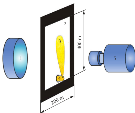
Figure 2. Optical measurement scheme and screen design: 1 – lamp; 2 – scattering screen; 3 – fuel jet; 4 – nozzle; 5 – high-speed video camera
