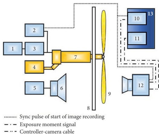
Figure 1. Schematic diagram of a high-speed video shooting stand for determining the parameters of a fuel jet: 1 – electronic engine control unit; 2 – synchronization devices; 3 – control block; 4 – fuel tank; 5 – power supply unit; 6 – light source; 7 – nozzle; 8 – screen; 9 – fuel jet; 10 – ADC LA 1.5 PCI; 11 – controller board; 12 – high-speed video camera “Videosprint”; 13 – PC
