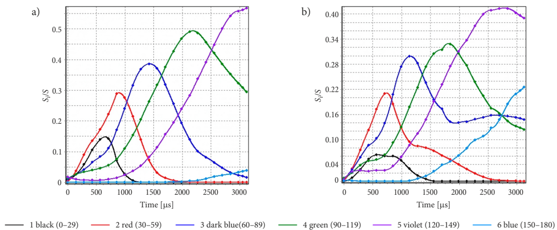
Figure 5. The structure of the fuel jet in CR system: a – DF; b – RME
