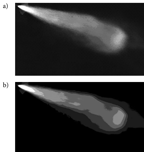
Figure 3. Fragments of recording the image of the fuel atomization process (image inverted): a – initial image (exposure time 35.5 \mu s); b – brightness zones, allocated by the computer program on the image using the threshold segmentation method
