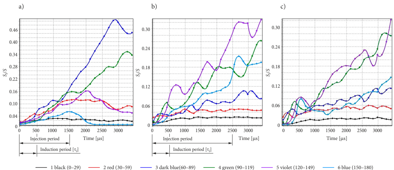
Figure 6. Fuel jet dynamics in the CDS system during injection: a – DF (26 °C); b – RO (26 °C); c – RO (65 °C)
