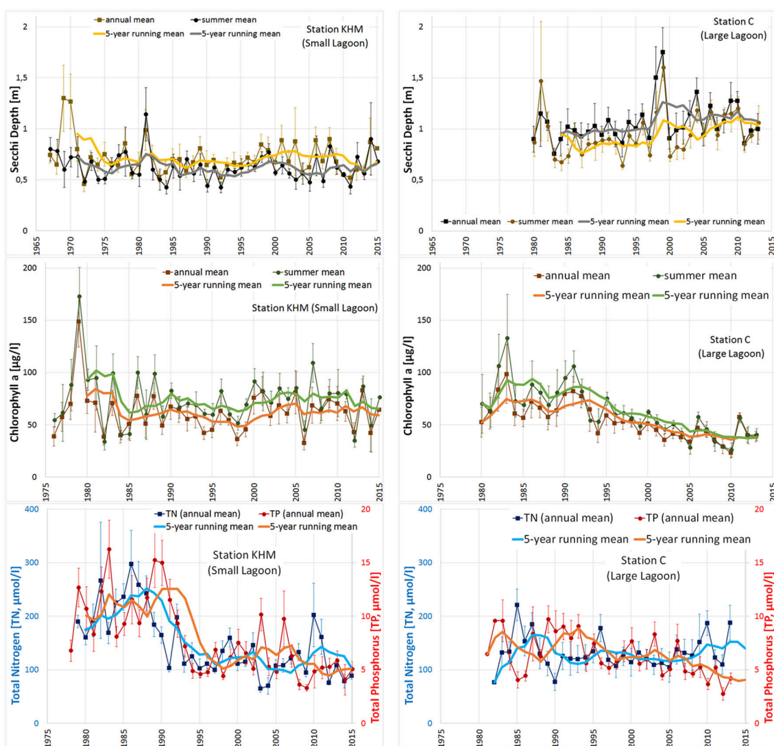
FIGURE 4 | Long-term time series of water quality parameters Secchi depth (m, upper panel), chlorophyll-a ( \mu\text{g/l} , middle) and TN & TP concentrations ( \mu\text{mol/l} , lower panel) together with standard errors and 5-year running means at the central stations of Small Lagoon (KHM, left column) and Large Lagoon (station C, right column). Summer period refers to May–September.
