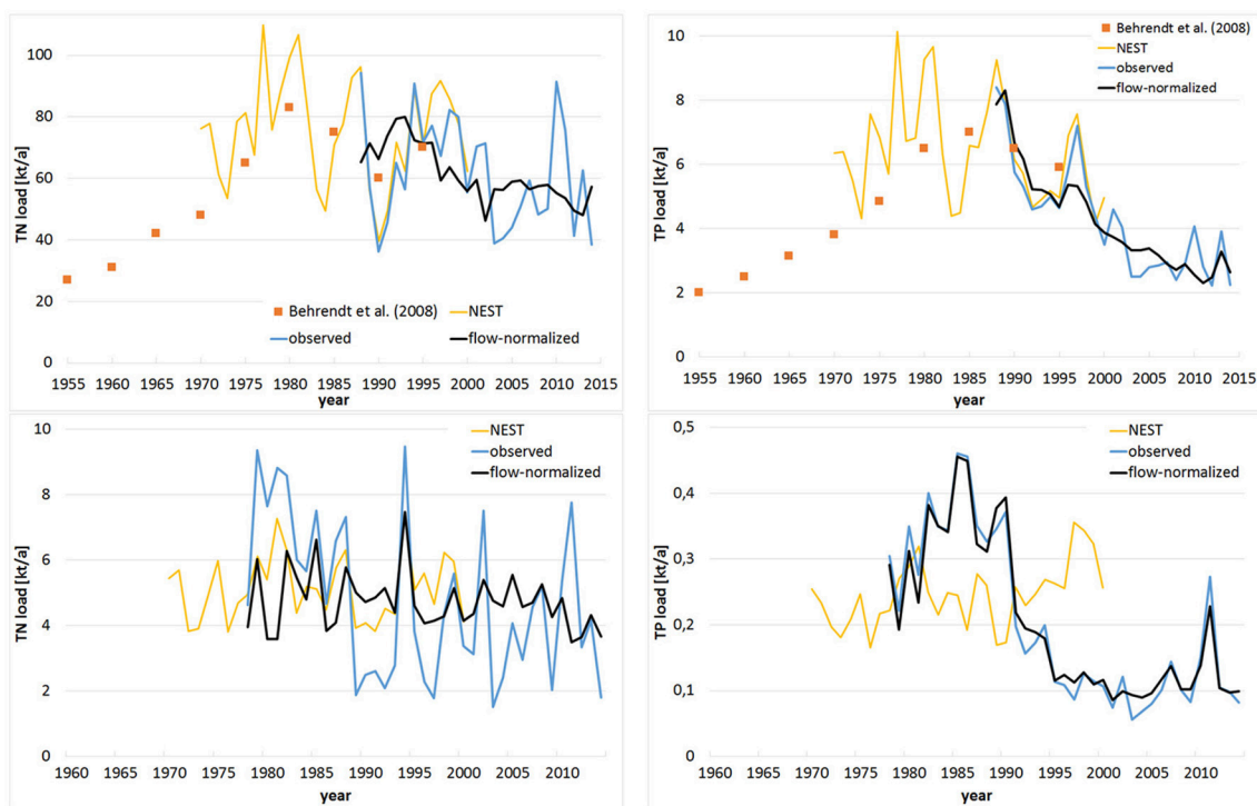
FIGURE 3 | Annual total nitrogen (TN) and total phosphorus (TP) loads discharged by Oder ( Upper ) and summed for Peene, Uecker and Zarow ( Lower ) based on observations (blue) and flow-normalization (black); supplemented by reconstructed loads from Baltic Nest Institute (yellow; Wulff et al., 2013) and Behrendt et al., 2008 (orange, only for Oder).
