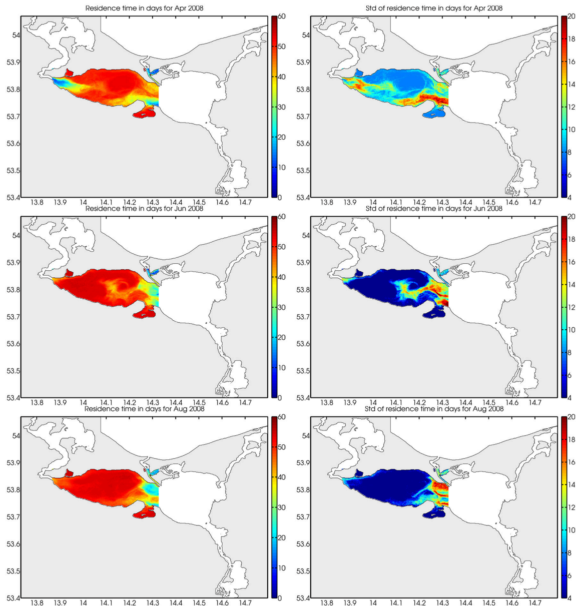
FIGURE 9 | Water residence times in Small Lagoon in April, June and August 2008 ( Left ) and their standard deviations ( Right ) calculated using ERGOM-GETM. Small Lagoon is always characterized by residence times near to the maximal value (the particle were only followed for 60 days).
