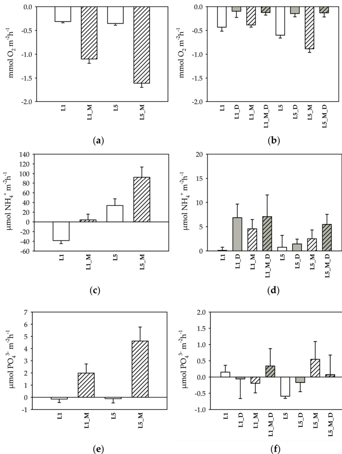
Figure 2. Dark net fluxes of O_2 (a,b), NH_4^+ (c,d), PO_4^{3-} (e,f) at day 5 (a,c,e) and at day 33 (b,d,f). Mean fluxes and standard error ( n = 10 at day 5 and n = 5 at day 33) of each condition are reported. All fluxes are expressed in \mu mol m^{-2} h^{-1} or mmol m^{-2} h^{-1} . White bars represent the permanently submerged condition, grey bars represent dried conditions and hatched bars represent conditions with macrofauna.
