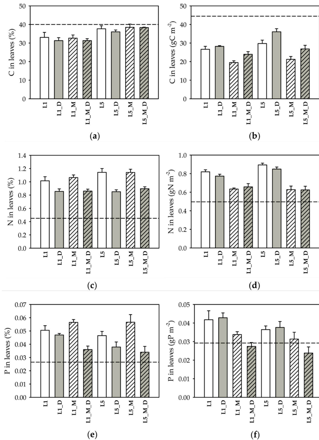
Figure 4. C, N and P percentage (a,c,e) and content (b,d,f) in the residual litter at the end of the experimental period. Mean \pm standard error ( n = 5 ) are reported. White bars represent the permanently submerged condition, grey bars represent dried conditions and hatched bars represent conditions with macrofauna. The horizontal dashed line is the reference value of the average C, N, P percentage and content in leaves at the beginning of the experiment.
