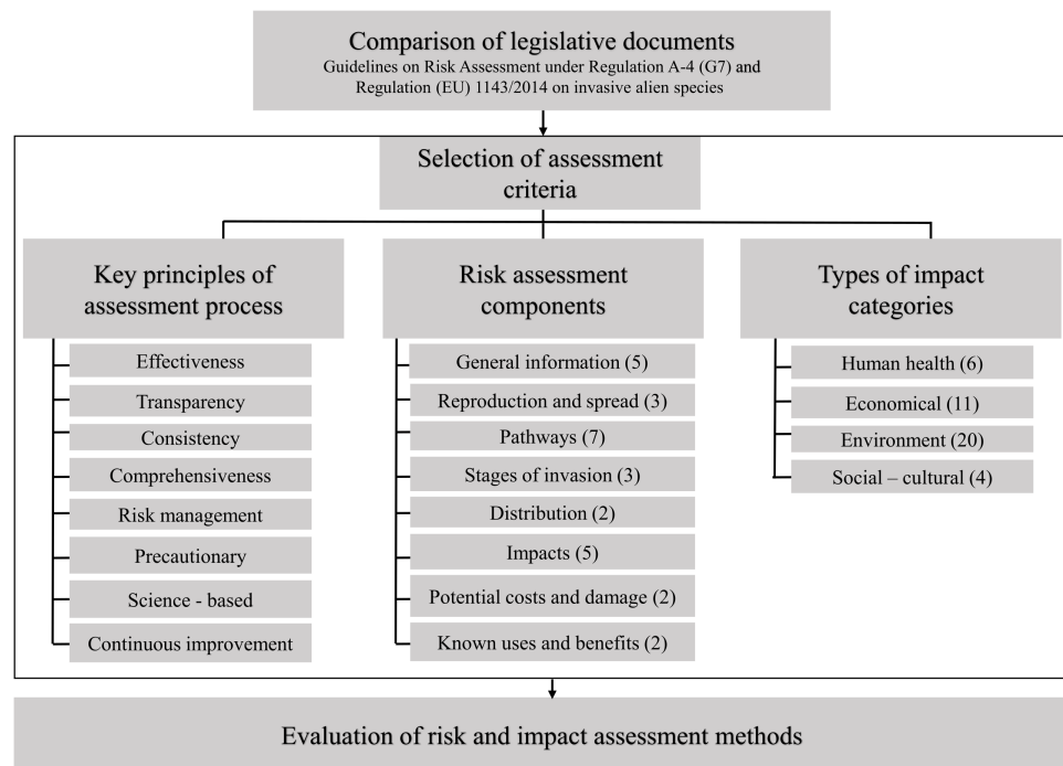
Figure 1 A stepwise process of the evaluation of bioinvasion risk and impact assessment methods: comparison of legislative documents, selection of criteria and evaluation. The number of elements in risk assessment components and categories in types of impact is given in brackets (listed in Tables S1 and S2, accordingly).
