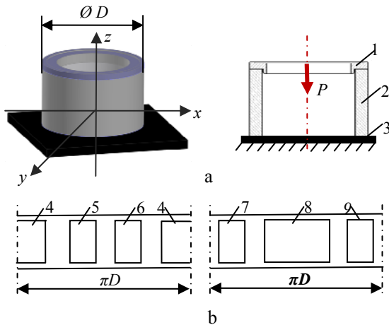
Fig. 2 Piezoceramic cylinder with a steel ring: a) general scheme, b) evolutes of a cylindrical inner and outer surfaces (single phase). 1 – steel ring, 2 – piezoelectric cylinder with electrodes formed on the outer and inner surfaces of the cylinder, 3 – vibrations depressant substance, 4-9 – electrode configurations
