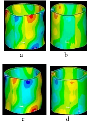
Fig. 3 Vibration of cylindrical actuator under 3-phase excitation voltage at four time steps: a) t = 0 ; b) t = \frac{1}{2} \frac{\pi}{\omega} ; c) t = \frac{\pi}{\omega} ; d) t = \frac{3}{2} \frac{\pi}{\omega}
