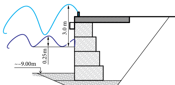
Fig. 6. The average annual height of waves for the period of 1999–2007 at the berths of the Port of Klaipėda
