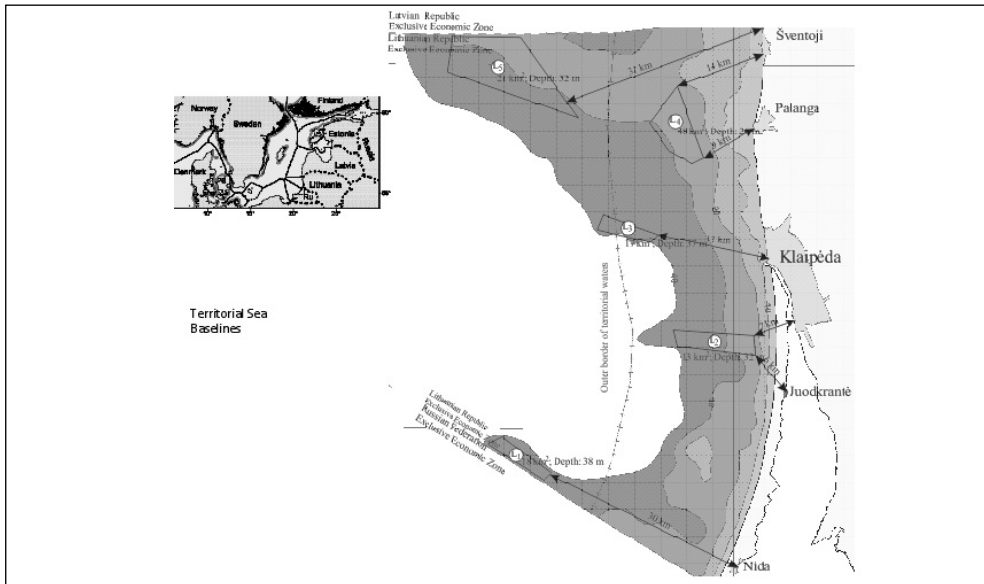
Fig. 1: Preliminary layout of the wind farms
