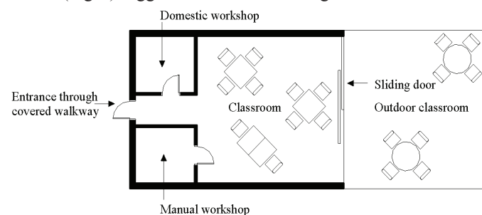
Fig. 2. Activity classroom by R. Neutra, 1935 [Scheme: G. Brukštutė].
