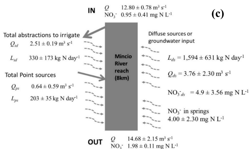
Figure 6. Nitrate and water budgets for the three reaches of Adda, Oglio, and Mincio rivers crossing the spring belt. Summer N budget were performed for the 18 km long Adda River reach (a), the 19 km long Oglio River reach (b), and the 8 km long Mincio river reach (c). River discharge ( Q ) and the nitrate concentration ( \text{NO}_3^- -N) are reported for the reach extremes (IN and OUT), while the discharge ( Q ) and the N load ( L ) are indicated for irrigation abstractions ( id ), point sources ( ps ), and diffuse sources ( ds ). From the nitrate and the water budgets, it was possible to estimate the \text{NO}_3^- concentrations of the diffuse inputs ( \text{NO}_3^-_{ds} ), which were compared to the \text{NO}_3^- concentrations in spring water from the measured data.
