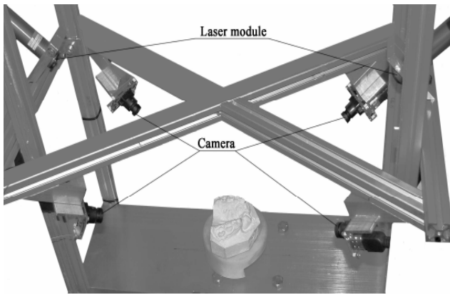
Fig. 1. System setup
