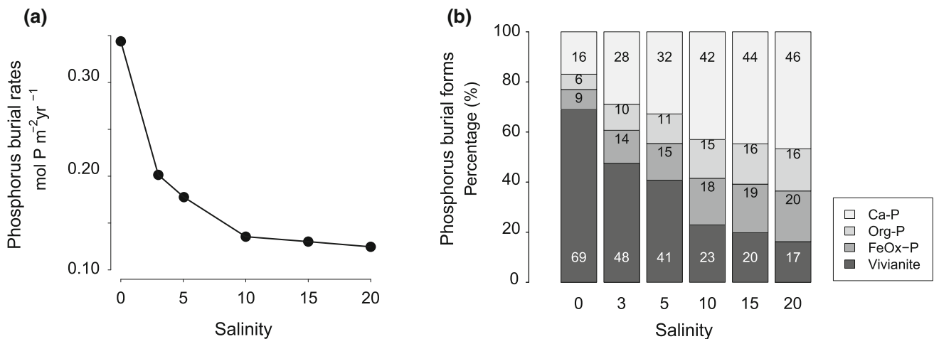
Fig. 5 Results of a sensitivity analyses of a reactive transport model for a site in the coastal zone of the Bothnian Sea illustrating the role of salinity in controlling P burial in the region (Lenstra et al. 2018)
