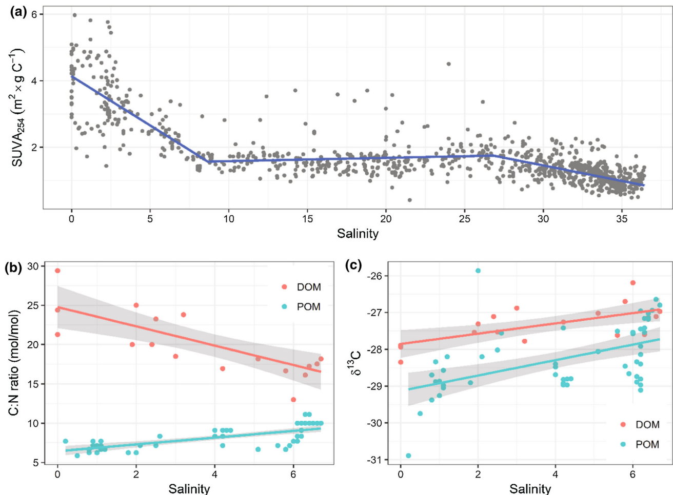
Fig. 6 Changing organic matter characteristics along the salinity gradient: a DOC-specific UV absorbance (SUVA 254 ), b C:N ratio and c stable isotope \delta^{13}\text{C} values in dissolved and particulate organic matter pools. Redrawn from Massicotte et al. (2017) (a), and Jilbert et al. 2018 (b, c)
