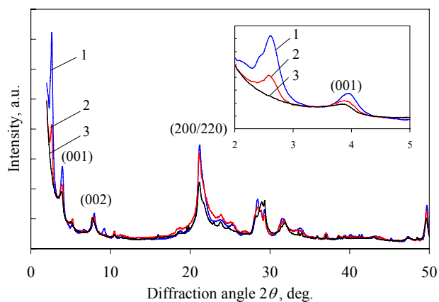
Fig. 4. X-ray diffraction patterns of organically modified sodium substituted gyrolite. Modification temperature: 1 – 80 ^\circ\text{C} , 2 – 100 ^\circ\text{C} and 3 – 120 ^\circ\text{C}
