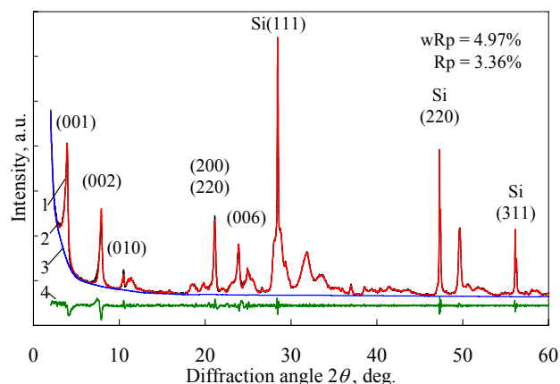
Fig. 1. The powder X-ray diffraction patterns of pure synthetic gyrolite after the final Le Bail's fitting: 1 – the observed scattered intensity ( Y_i^{\text{obs}} ), 2 – the calculated intensity ( Y_i^{\text{calc}} ), 3 – background and 4 – the difference between the observed and calculated intensities ( Y_i^{\text{obs}} - Y_i^{\text{calc}} )
