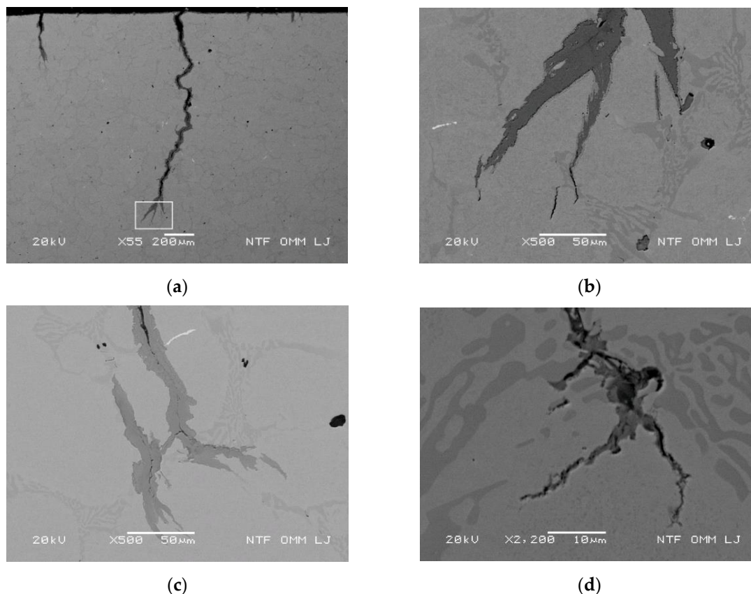
Figure 13. Influence of oxidation on crack branching: (a) crack exceeding 1300 μm with marked area of subfigure b, (b) primary crack branching and individual approaches of oxide branches to internal cracks, (c) branching of the primary crack by oxidation based on low thermal stresses and growth in area with depleted Cr content and (d) branching of the primary crack in the preferred oxidation direction and growth towards areas with depleted Cr content in a narrow band adjacent to the eutectic.
