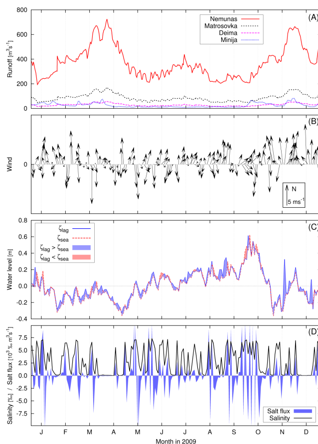
Fig. 5. Time series of (A) fresh water discharge into the lagoon, (B) wind speed vector azimuth in the northern part of the lagoon, (C) modelled water level in the open shelf in front of the lagoon (red dotted line) and in the northern part of the lagoon (blue continuous line), (D) modelled salt flux through cross-section S5 (blue band; positive value indicates flow toward lagoon and negative value indicates flux seawards) and depth averaged salinity in the northern part of the lagoon (black line).
