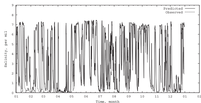
Fig. 2. Time-series of observed and modelled surface salinity in the Klaipėda harbour.
