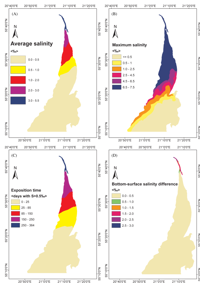
Fig. 4. Spatial distribution in the northern part of the Curonian Lagoon of (A) annual average of vertically-averaged salinity, (B) yearly maximum of vertically-averaged salinity, (C) number of days per year when vertically-averaged salinity stays greater than 0.5 ‰, (D) difference between annual average of surface and near bottom layer salinity.
