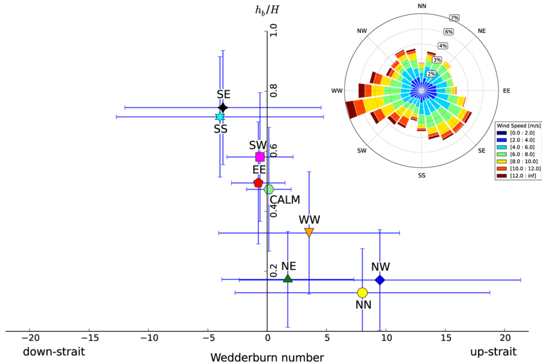
Fig. 10. Flow-regime diagram to classify the effect of the wind on stratification in the Klaipėda Strait. The y-axis is the ratio of buoyancy layer depth ( h_b ) to total water depth ( H ); the x-axis is the Wedderburn number ( W ). Positive is up-strait and the blue error-bars indicate the standard deviation of W . Symbols identify the mean values of each sub-sample based on the wind direction (from NN, NE, EE, SE, SS, SW, WW and NW) and the no-wind situation (CALM; sub-sample of cases with wind intensity lower than 3 \text{ m s}^{-1} ). In the upper right panel the wind rose obtained from HIRLAM model results for the Klaipėda Strait is shown.
