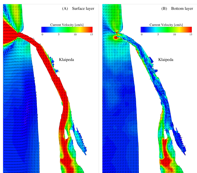
Fig. 6. Maps of yearly averaged modelled surface (A) and bottom (B) currents in the Klaipėda Strait.
