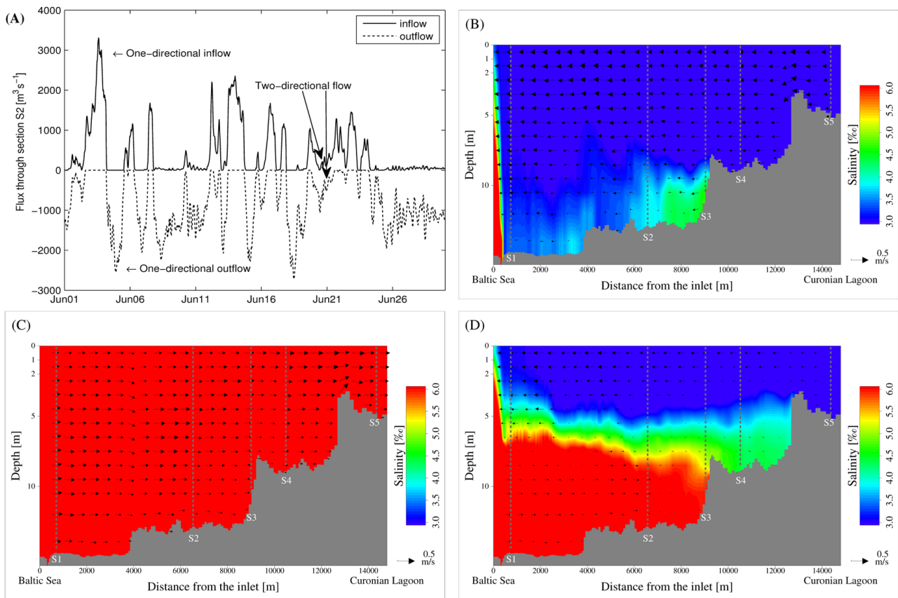
Fig. 7. Water flow through cross-section S2 in June 2009 ( (A) , continuous line for inflow and dotted line for outflow) and different flow regimes in the Klaipėda Strait: (B) unidirectional outflow, (C) unidirectional inflow, (D) two-layer flow. Grey dotted lines in panels (B) , (C) , (D) indicate the approximate location of cross-sections S1–S5.
