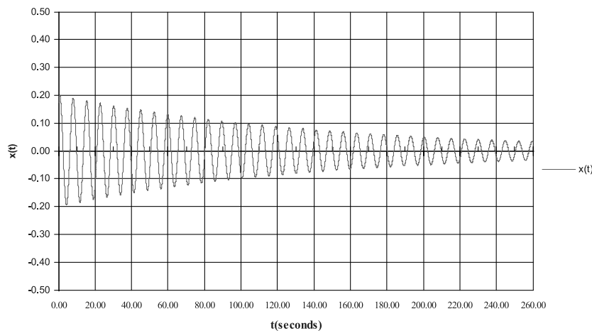
Fig. 2. The asymptotic stable solution received with the help of numerical method.
