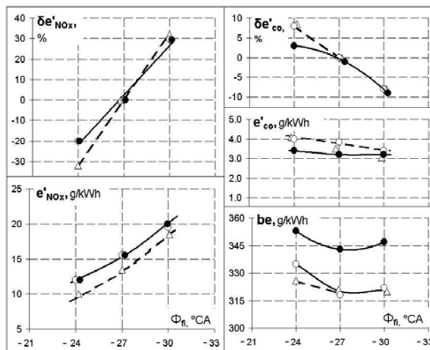
Fig 3. Influence of fuel injection phase of diesel engine A41 on ecological parameters ( n = 1750 rpm; p_{mi} = 0,68 MPa): ○— mineral diesel fuel; ●— biodiesel B100; △— biodiesel B30
