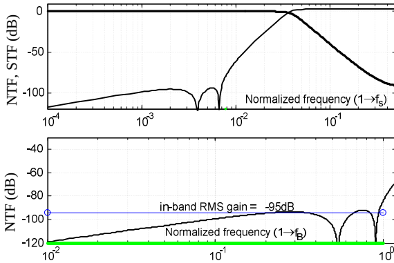
Fig. 8. Signal and noise transfer functions
