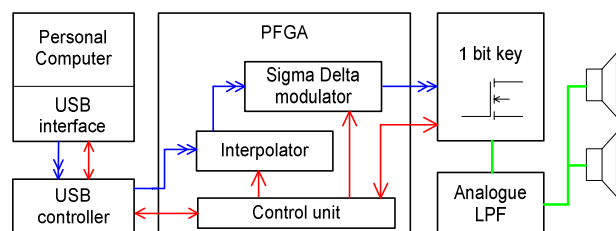
Fig. 1. Simplified structure of DAC on FPGA
