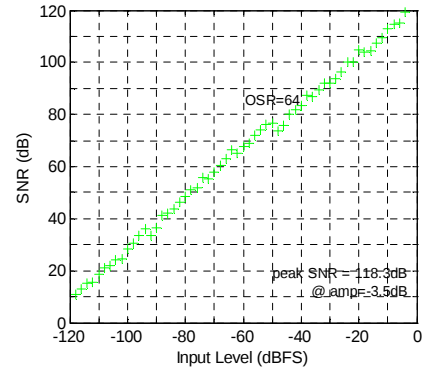
Fig. 9. Signal-to-noise ratio
