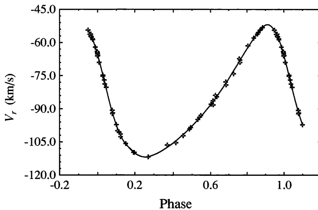
Fig. 3. Radial velocity curve.
