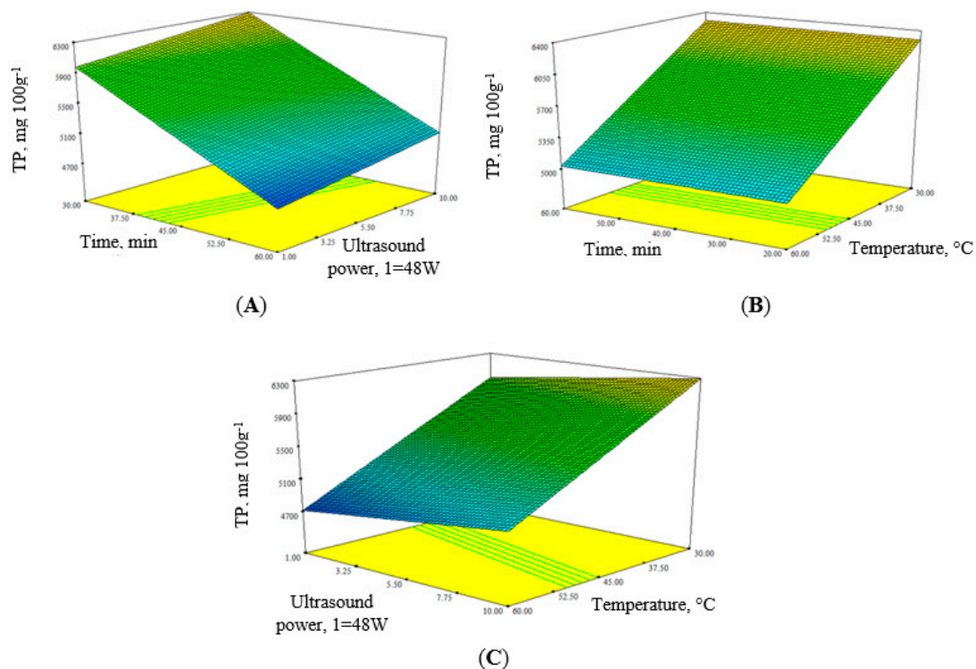
Figure 1. Response surfaces plots for total phenols (TP) in Japanese quince fruit, in the function of ultrasound power, extraction time, and temperature. (A)—Extraction time and ultrasound power; (B)—extraction time and temperature; (C)—extraction temperature, and ultrasound power.
