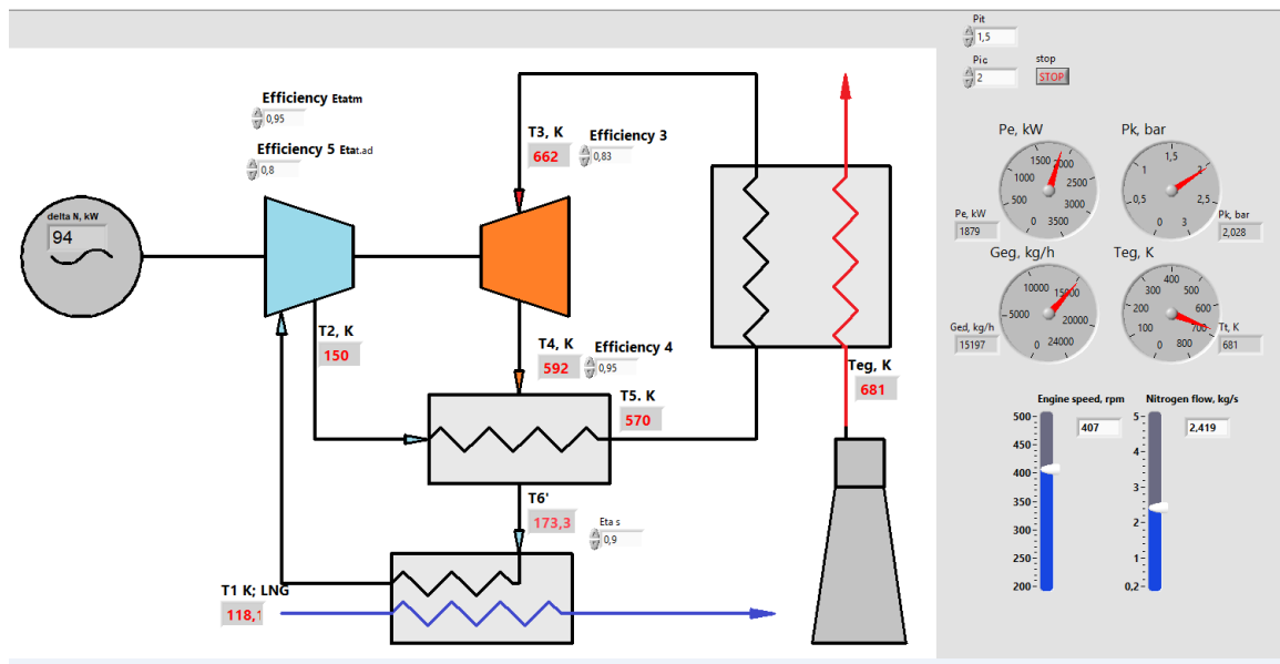
Figure 3. Fragment of an LNG ship power plant cogeneration cycle simulator.
