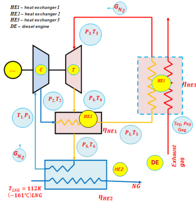
Figure 1. Principal scheme of liquefied natural gas (LNG) ship's power plant cogeneration cycle (T: turbine; C: compressor; E: engine; HE i : heat exchanger).
