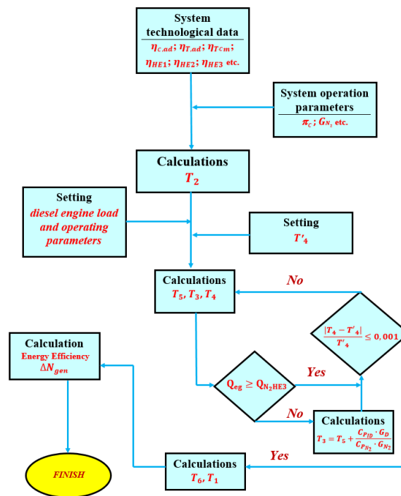
Figure 2. Algorithm for the simulation of the LNG ship's power plant cogeneration cycle.
