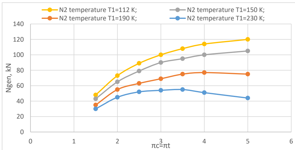
Figure 6. Effect of technological system parameter \pi_C = \pi_T on N_{gen} .
