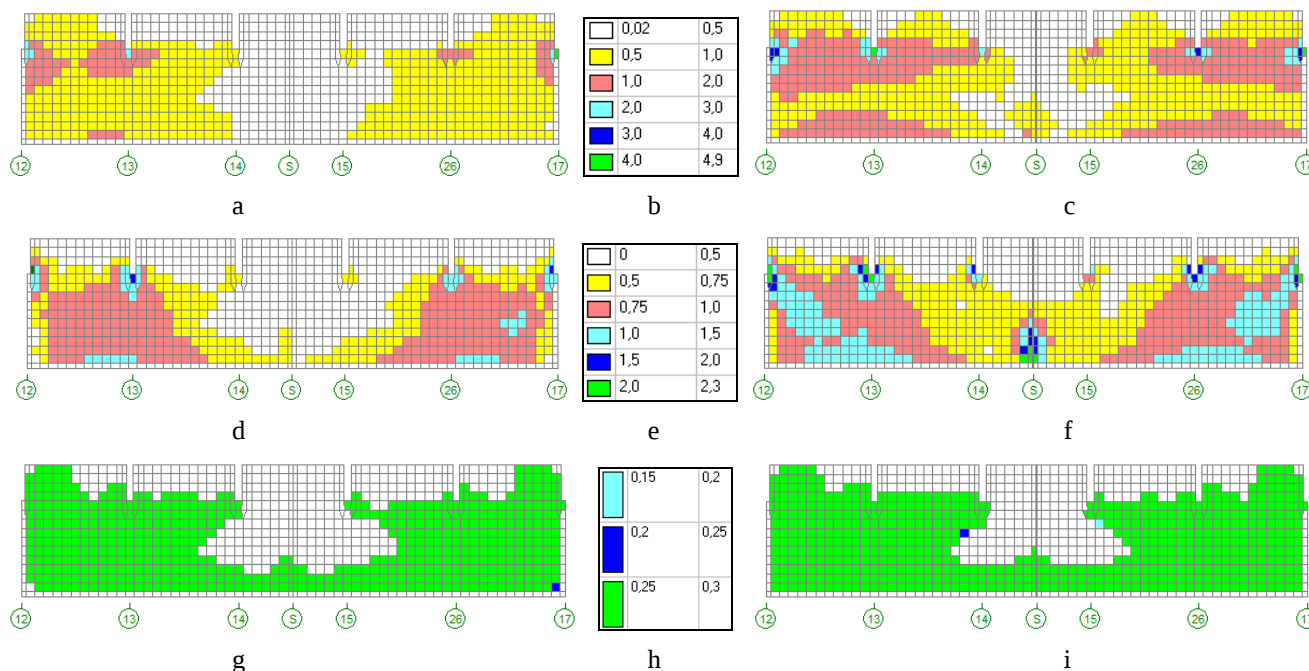
Fig. 15 The reinforcement in external wall of sector III on axis “B”, axes from “12” to “17”, of storage facility: a – results from ordinary combinations; b – X-axis intensity (%), scale of colours; c – custom combinations; d – results from ordinary combinations; e – Y-axis intensity (%), scale of colours; f – custom combinations; g – results from ordinary combinations; h – crack widths (mm), scale of colours; i – custom combinations
