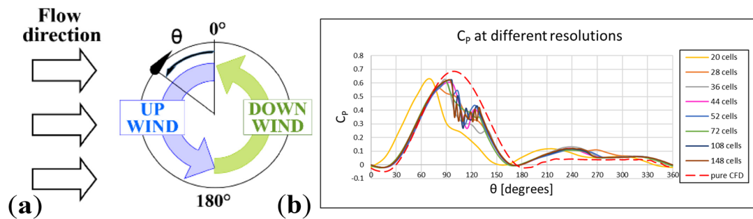
Figure 5. (a) Scheme of upwind and downwind path; (b) C_p for a single blade at different resolution.
