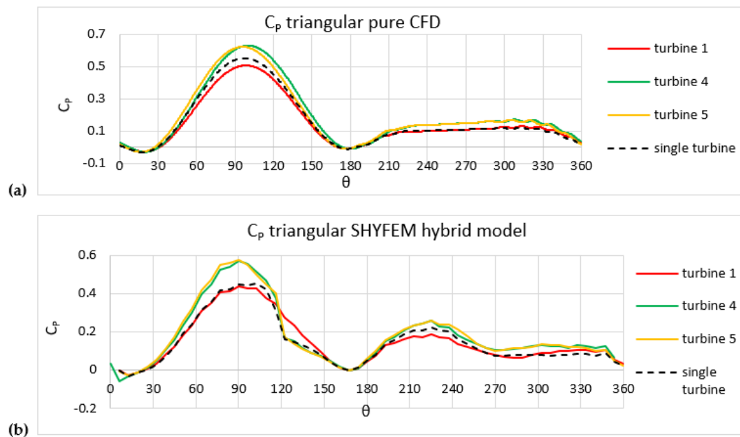
Figure 18. C_p for the triangular triad both for the pure CFD (a) and SHYFEM hybrid model (b).
