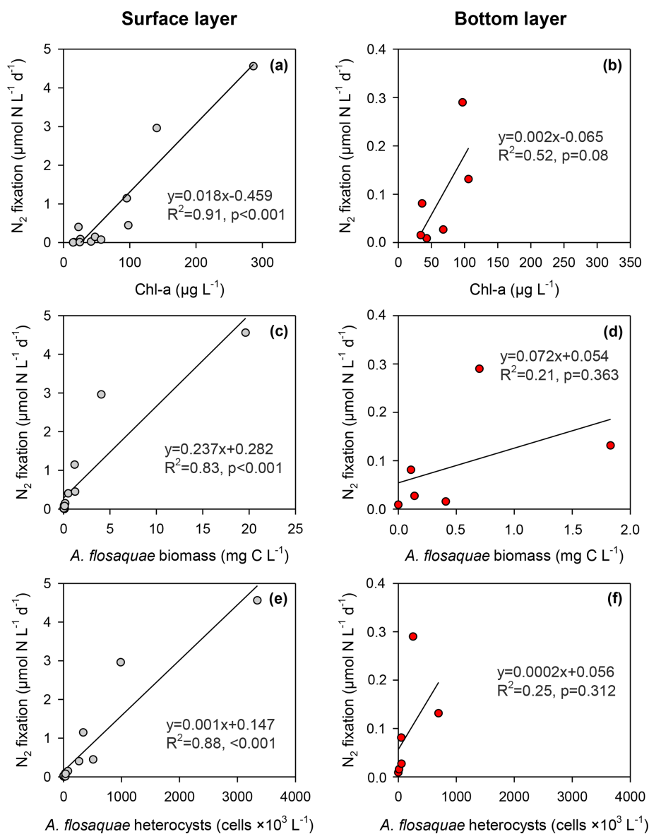
Figure 7. Relationships between N 2 fixation and in situ measured chlorophyll a ( a , b ), A. flosaquae biomass ( c , d ) and their heterocysts ( e , f ) in surface (northern and central sites, left panels) and bottom (central site, right panels) layers of the Curonian Lagoon during April–September 2018.
