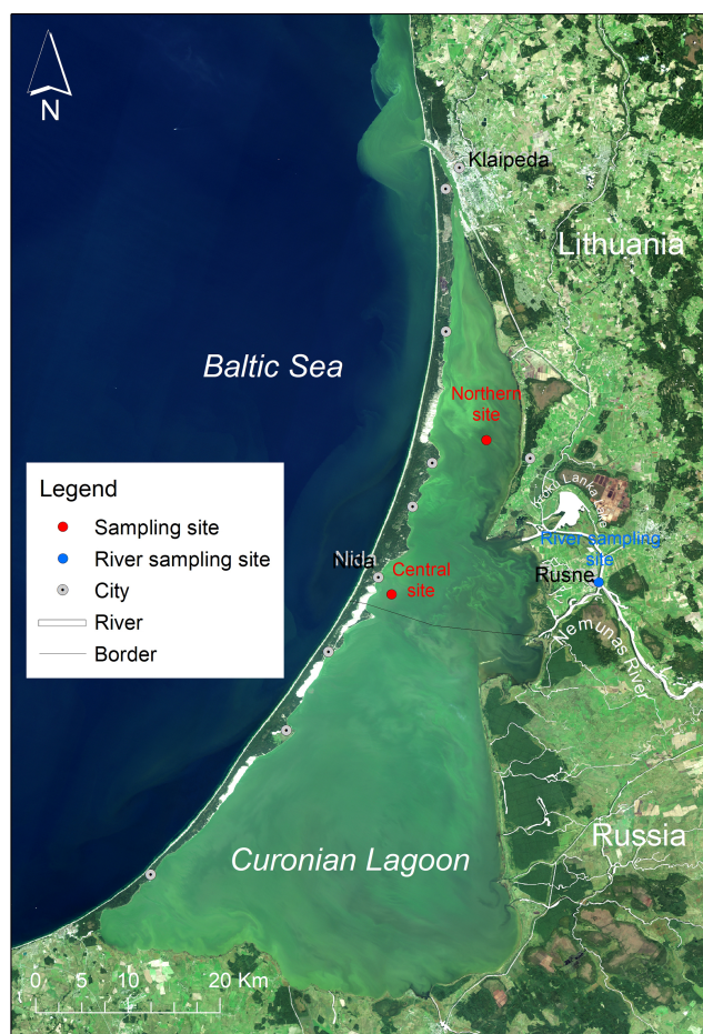
Figure 1. Satellite image by OLI/Landsat-8 (18 September 2014) showing summer blooms in the Curoonian Lagoon with the sampling sites (red circles) representing the northern and south-central regions, and monitoring site at the Nemunas river (blue circle). LT = Lithuania, RUS = Russia, and the black line indicates a border between the two countries.
