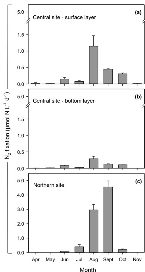
Figure 5. Rates of N 2 fixation at central (a, b) and northern (c) sites in the Curonian Lagoon in 2018 (data are mean values and standard error based on three replicates).
