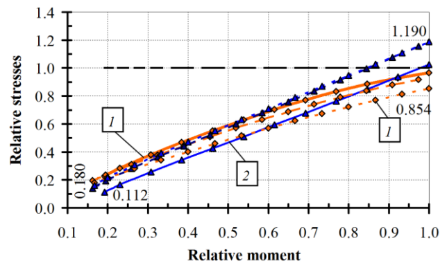
Fig. 9 The variation of relative stresses, depending on the relative bending moment: 1 – the top point of concrete; 2 – reinforcement
