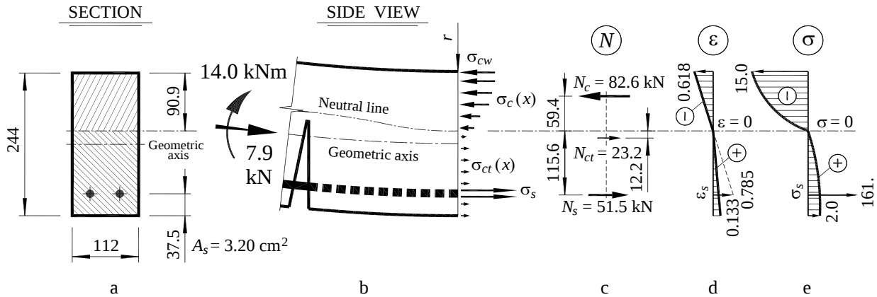
Fig. 6 The calculation scheme and results of the beam cross section in the middle between cracks: a) section view; b) side view; c) cross-sectional forces; d) diagram of strains; e) diagram of stresses
