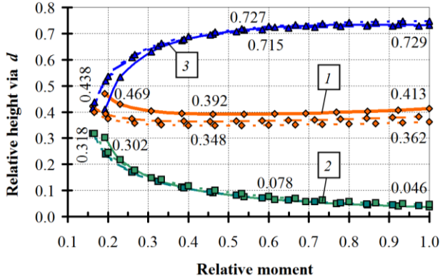
Fig. 7 The variation of relative cross-sectional height of zones, depending on the relative bending moment: 1 – compressive layer; 2 – tensile layer; 3 – crack deep
