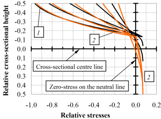
Fig. 10 The distribution of relative stresses in the direction of the cross-sectional height, when the bending moment 5.0, 8.0, 14.0, 20.0 and 26.0 kNm: 1 – black lines mark the section with cracks, 2 – gray lines denote the whole section
