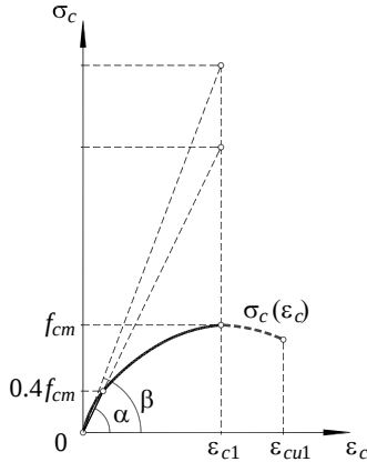
Fig. 2 The compressive concrete stress/strain relation from the design code EN 1992
