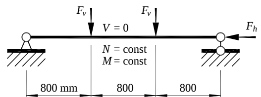
Fig. 4 The testing scheme of beams
