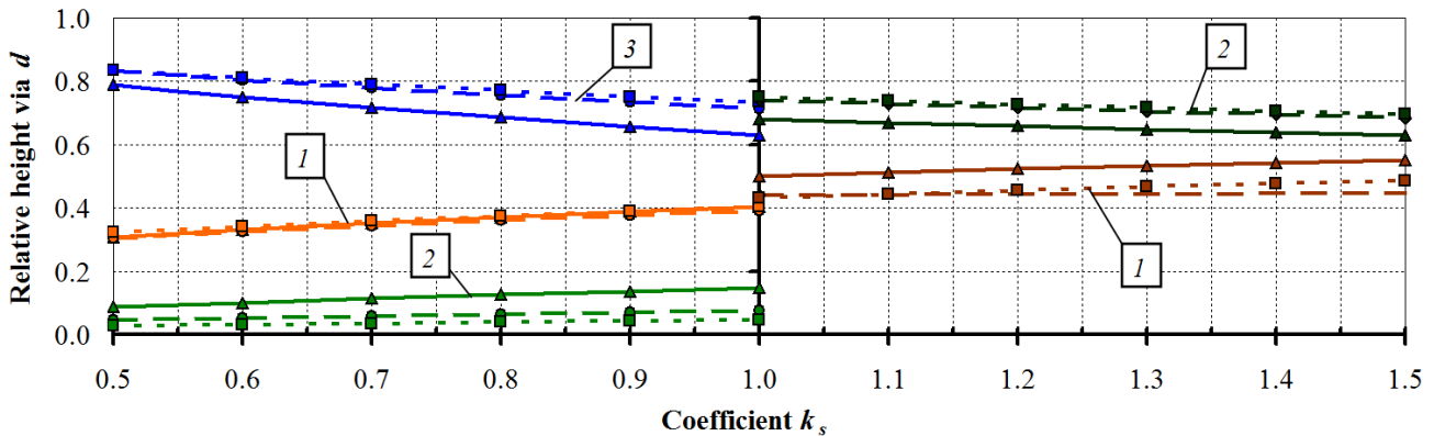
Fig. 11 The variation of the relative cross-sectional height, depending on the coefficient k_s (7th beam group): 1 – height of the compressive layer; 2 – height of the tensile layer; 3 – the crack deep
