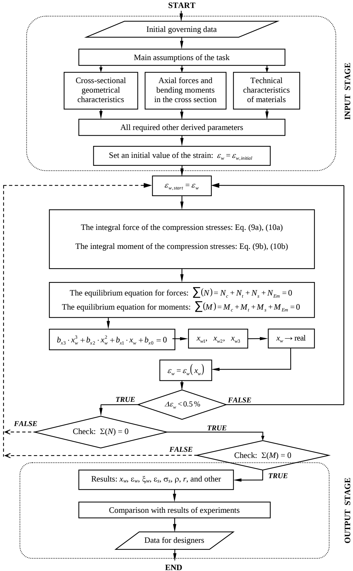
Fig. 3 The algorithm of the mechanical state analysis of a reinforced beam by the ZI method
