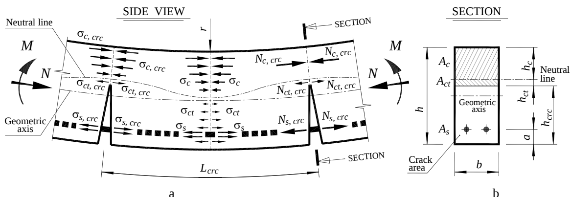
Fig. 1 A scheme of a beam with cracks under compression with bending: a) side view; b) section view
