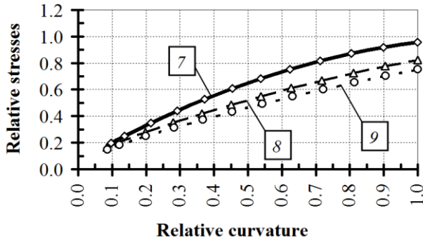
Fig. 12 The variation of relative stresses via the relative curvature (the marks show the numbers of beam groups)
