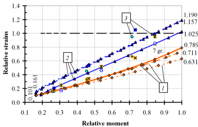
Fig. 8 The variation of relative strains, depending on the relative bending moment 1 – the top point of concrete; 2 – reinforcement; 3 – experimental data
