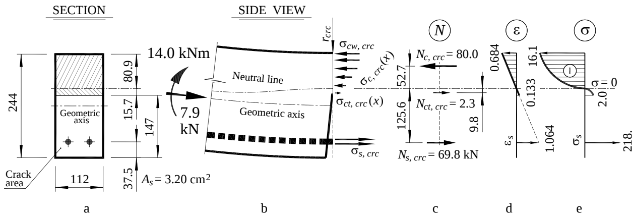
Fig. 5 The calculation scheme and results of the beam cross section at the crack: a) section view; b) side view; c) cross-sectional forces; d) diagram of strains; e) diagram of stresses
