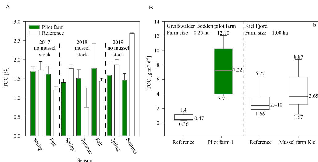
Figure 7 TOC of surface sediment and bio deposition rates within the pilot farm 1. (A) Surface sediment TOC at the pilot farm 1 (green) compared to reference measurements (white) from 2017 to 2019 divided by seasons and presence of mussel stock. (B) TOC sedimentation rate in the water column in pilot farm 1 (green) and at a reference site (white). For comparison, results from the commercial mussel farm in Kiel are added.
