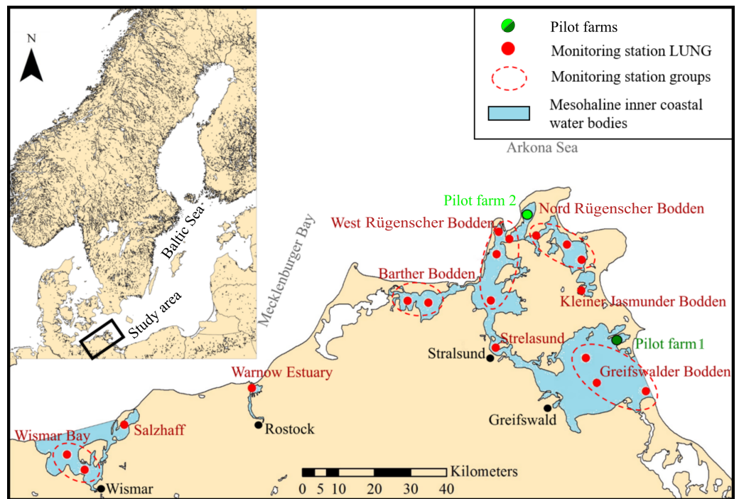
Figure 1 Map of the study site. Mesohaline inner coastal water bodies (blue areas, labeled in red) including monitoring stations of the State Agency for Environment, Nature Conservation and Geology Mecklenburg-Vorpommern (LUNG) (red dots) providing environmental data for every water body in the study area (where multiple measuring stations occur, data of these stations are pooled (marked by a dotted line)). Green dots represent the two pilot mussel farms.
