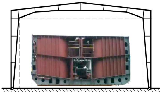
Fig. 3 The mobile frame over a ship block
