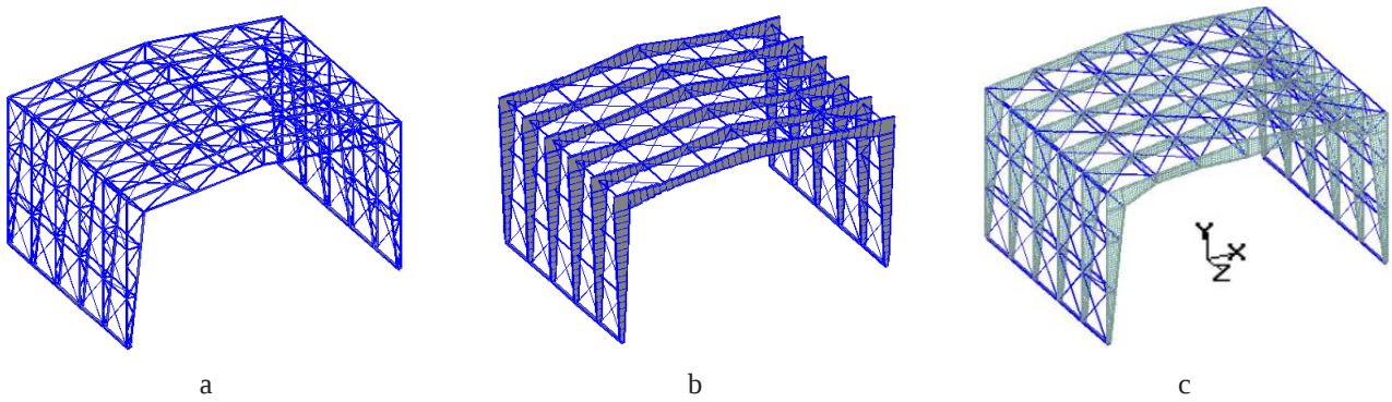
Fig. 7 A general views of FEM models: a – Truss 1D; b – Beam 1D; c – Plate 2D
