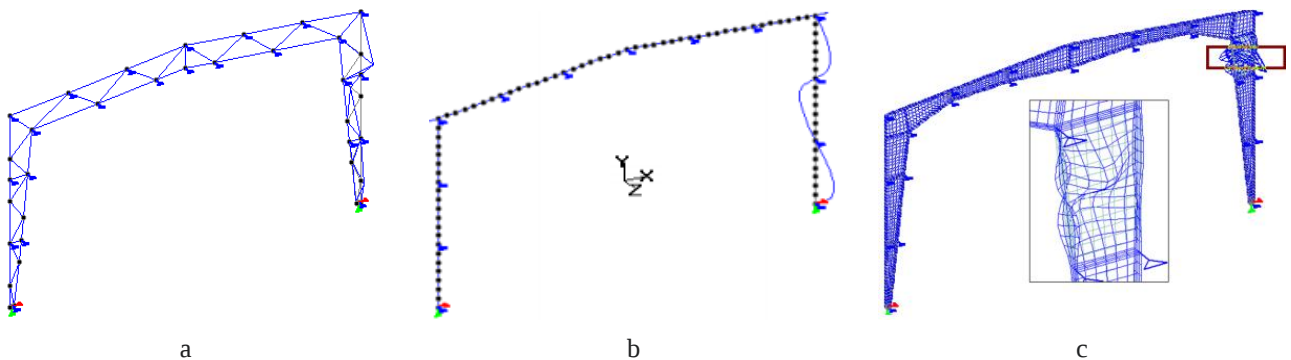
Fig. 8 The first buckling mode shape of the FEM frame: a – Truss 1D; b – Beam 1D; c – Plate 2D
