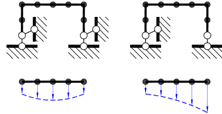
Fig. 4 Movement schemes of the mobile frame
