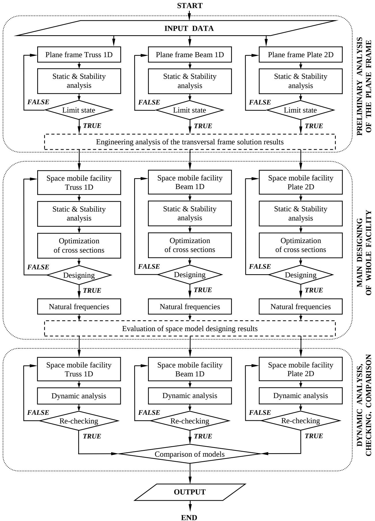
Fig. 6 The structural analysis algorithm of different types of the frames
