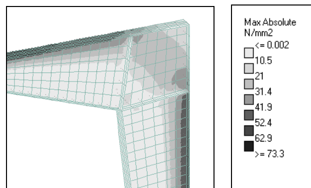
Fig. 10 The stress distribution in scheme Plate 2D at the column/beam joint
