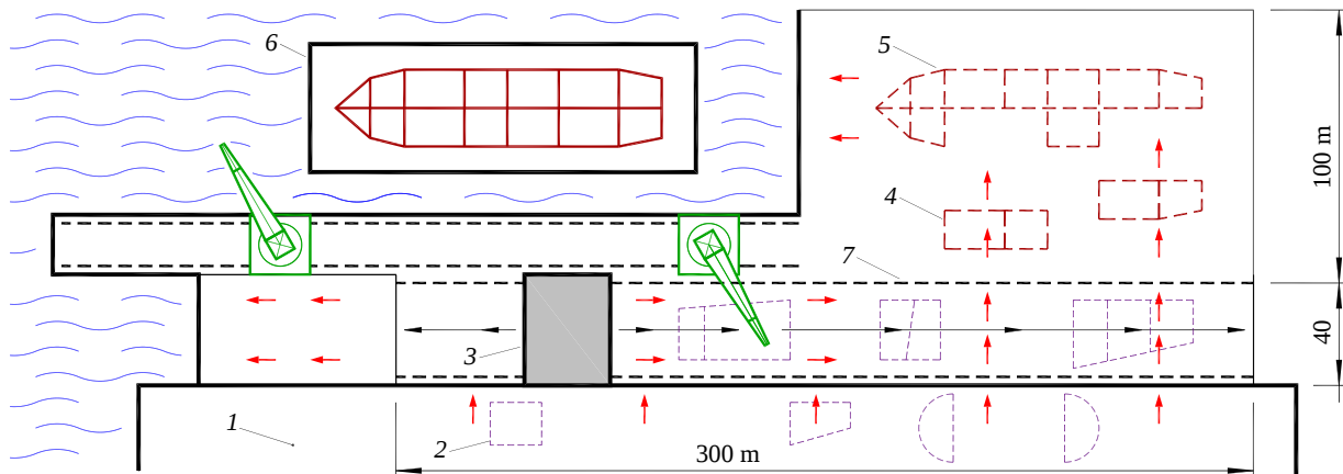
Fig. 5 The scheme of the open area for assembling: 1 – factory; 2 – block; 3 – mobile facility; 4 – superblock; 5 – ship hull; 6 – barge; 7 – railway
