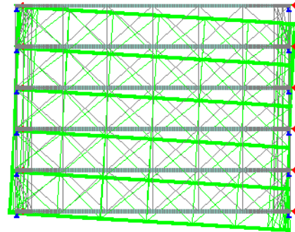
Fig. 9 Top view of deformation scheme Plate 2D, while one side is fixed
